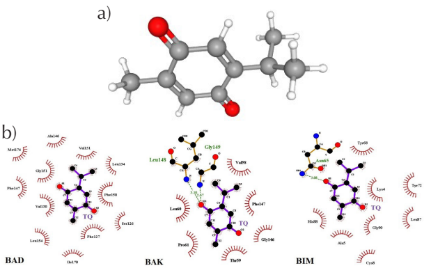
Figure 1. a) The Structure of TQ, b) Hydrogen and Hydrophobic Bonds Between TQ and Bonded Residues in Binding Sites.
