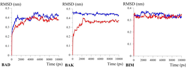
Figure 3. Root Mean Square Deviation (RMSD) for Bad, Bak, and Bim in complex with TQ. Blue line: simulation without TQ, Red line: simulation with TQ. Statistical analysis was done by independent samples t -test. Each point represents mean±SD. The difference between the red and blue lines was significant ( P<0.001 ).
