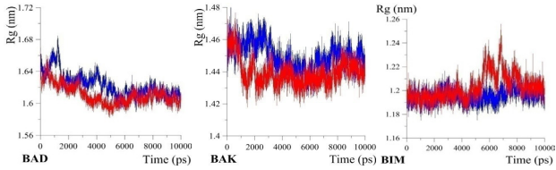
Figure 5. The Radius of Gyration (Rg) for Bad, Bak, Bim in Complex with TQ. Blue line: simulation without TQ, Red line: simulation with TQ. Statistical analysis was done by independent samples t -test. Each point represents mean±SD. The difference between the red and blue lines was significant ( P<0.001 ).
