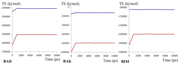
Figure 4. Total Energy (TE) for Bad, Bak, and Bim in Complex with TQ. Blue line: simulation without TQ, Red line: simulation with TQ. Statistical analysis was done by independent samples t test. Each point represents mean±SD. The difference between the red and blue lines was significant ( P<0.001 ).
